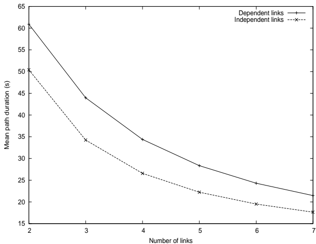
Figure 3: Mean path duration vs link count.
