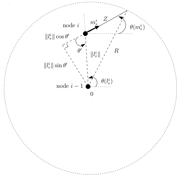
Figure 1: Link duration between two nodes with respect to the relative motion.
